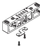
sub-base with open air supply and closed exhausts GP-6240 without electrical connection GP-6241 monostable GP-6242 bistable
